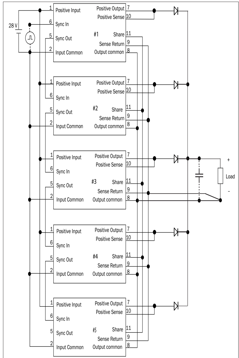
FIGURE 5: PARALLELING
