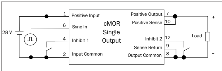
FIGURE 6: TYPICAL CONNECTIONS WITH SENSE PIN
