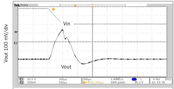
100 μs/div 50 to 15 V cMOR2805S STEP LINE RESPONSE
