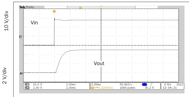
2 ms/div All combinations of line and load cMOR2805S START-UP RESPONSE
