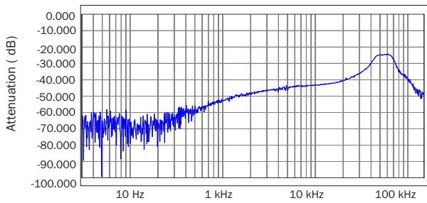
Frequency (kHz) cMOR2815D Audio Rejection
