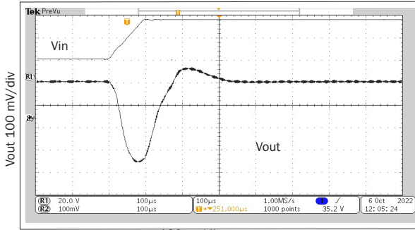
100 μs/div 15 to 50 V cMOR2805S STEP LINE RESPONSE
