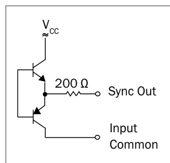
FIGURE 4: SYNC OUT
