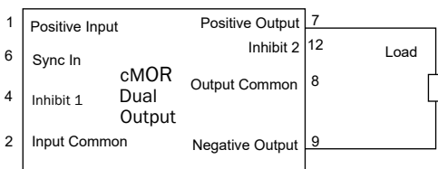
FIGURE 7: SPAN OUTPUT CONNECTION - DUAL MODEL
