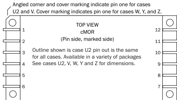
FIGURE 10: PIN OUT TOP VIEW
