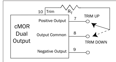
FIGURE 3: TRIM - DUAL
