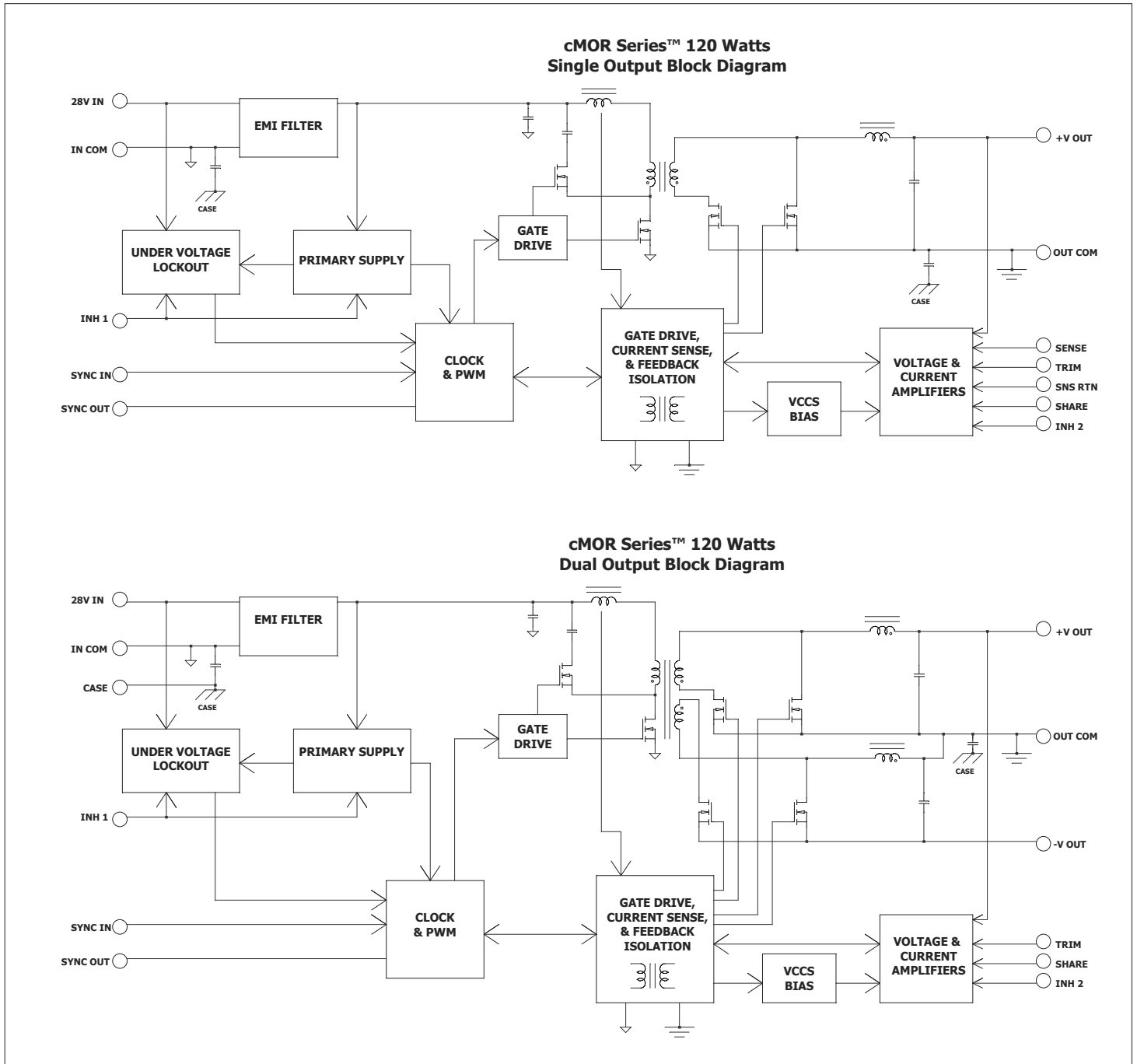
FIGURE 9: cMOR SINGLE AND DUAL OUTPUT BLOCK DIAGRAM
