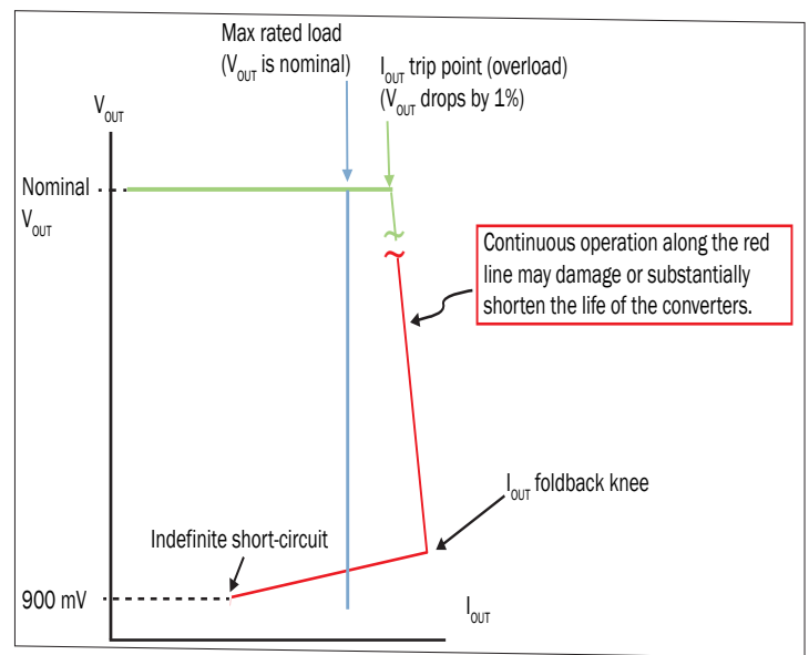
FIGURE 8: OUTPUT OVERLOAD AND SHORT-CIRCUITS PROTECTION
