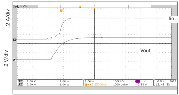
1 ms/div cMOR2805S INHIBIT RELEASE INRUSH CURRENT
