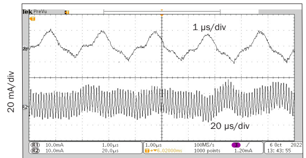
(PLACE HOLDER_PENDING) rMOR2815D Input Ripple Current (lin) FIGURE 28
