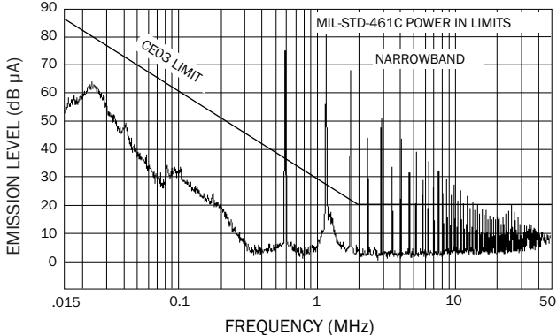
High power DC-DC converter without filtering.
