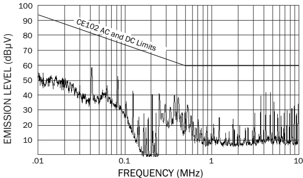
CE102: High power converter filtered with an FMCE-0528.
